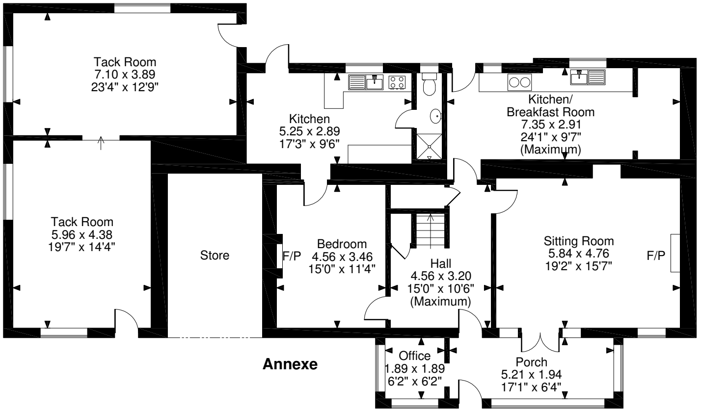
Ground Floor
