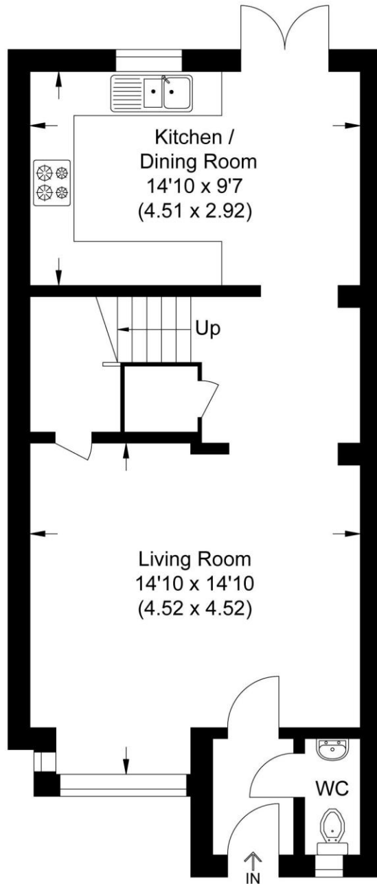
Ground Floor
