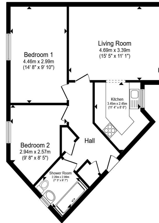
Floor Plan
