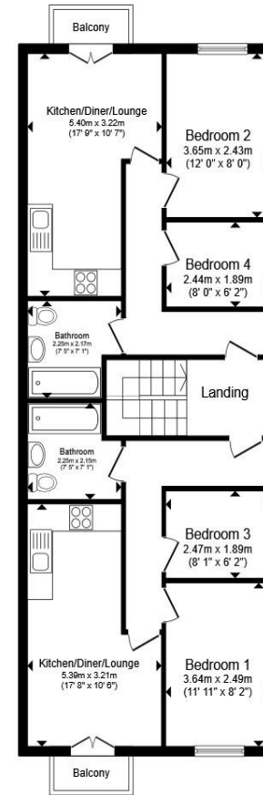
Second Floor
