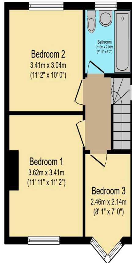
First Floor Floor area 38.1 m 2 (410 sq.ft.) approx
