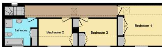
First Floor
