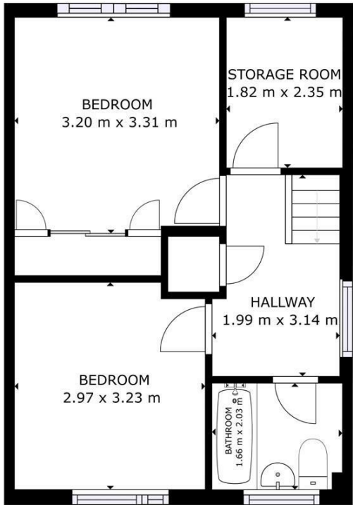
FLOOR 2
