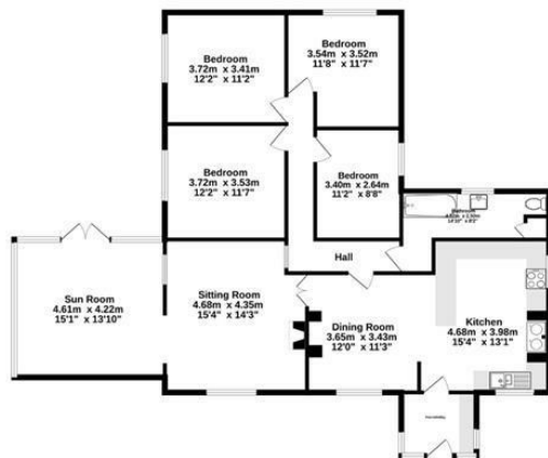
Ground Floor 134.8 sq.m. (1451 sq.ft.) approx.
