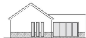
South facing elevation 1:100
