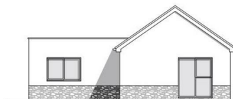
North facing elevation 1:100
